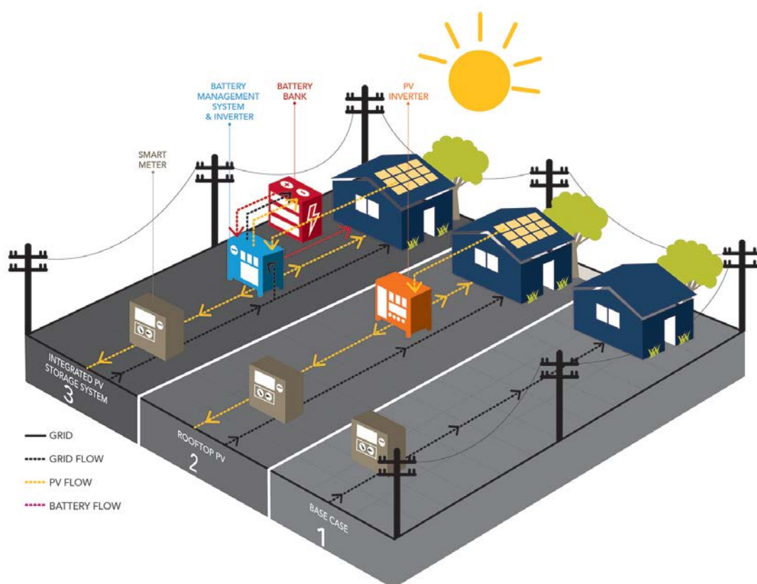
Figure 2 Residential IPSS system flow diagram
